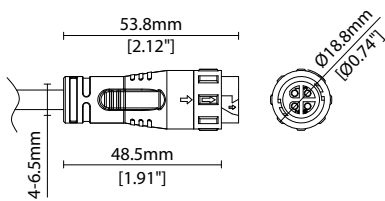
4 Pin RGB Female Connector IP67 (Premoulded)
