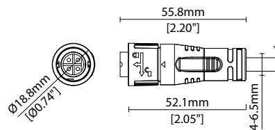
4 Pin RGB Male Connector IP67 (Premoulded)
